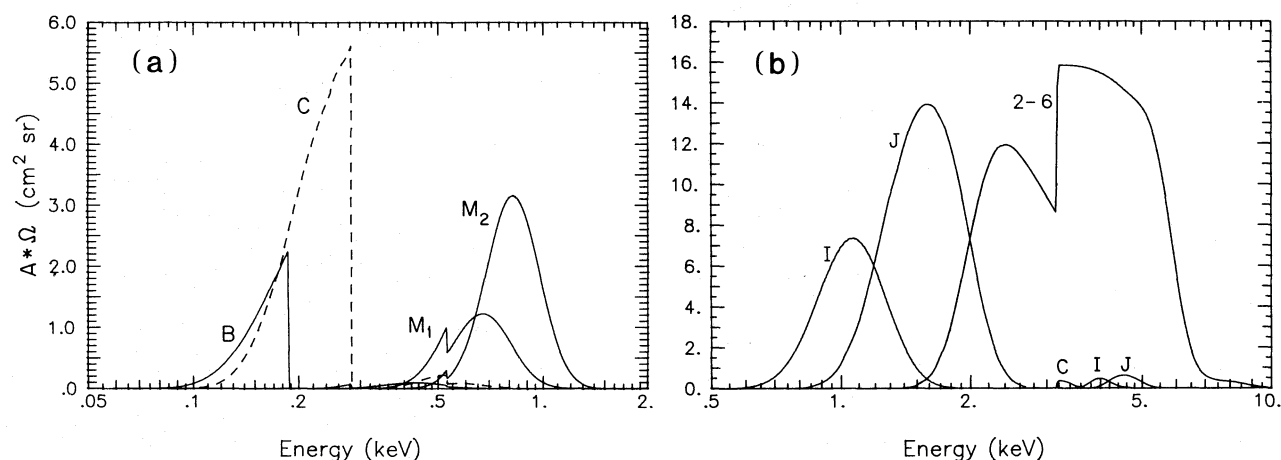
FIG. 1.—Net throughput band response functions. (a) B, C, M_1 , and M_2 bands. (b) I, J, and 2-6 keV bands. The B, M_1 , and M_2 bands have smaller responses above 3 keV due to argon fluorescent escape than that shown for C band.
