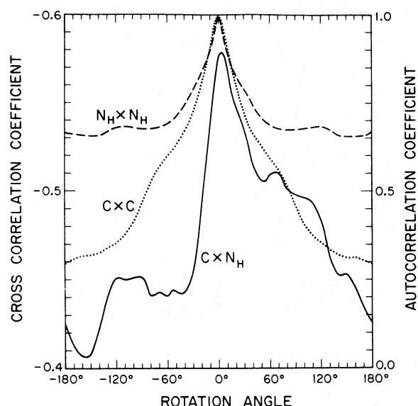
FIG. 12.—Change in correlation coefficient between C band X-ray intensity ( C ) and H I column density ( N_{\text{H}} ) as the H I distribution is rotated around the galactic polar axis with respect to the X-ray data. The cross-correlation coefficient is calculated as (\langle CN_{\text{H}} \rangle - \langle C \rangle \langle N_{\text{H}} \rangle) \times [(\langle C^2 \rangle - \langle C \rangle^2)(\langle N_{\text{H}}^2 \rangle - \langle N_{\text{H}} \rangle^2)]^{-1/2} using a 1.8 \times 1.8 grid. The autocorrelations for X-ray intensity and H I column density are shown, respectively, as dotted and dashed lines (right-hand scale).
